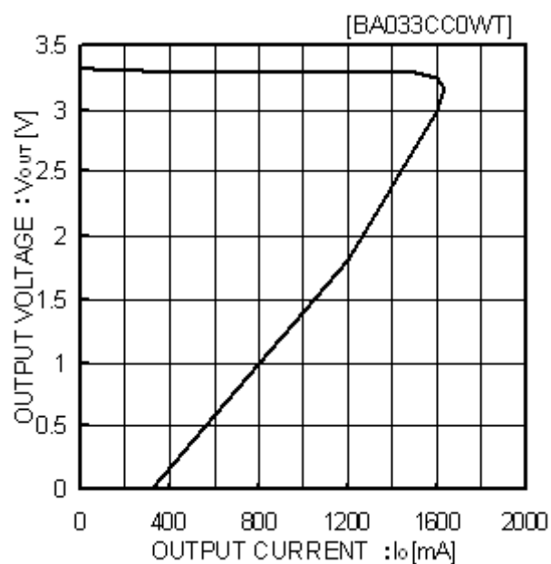
Fig.6 Load Stability
