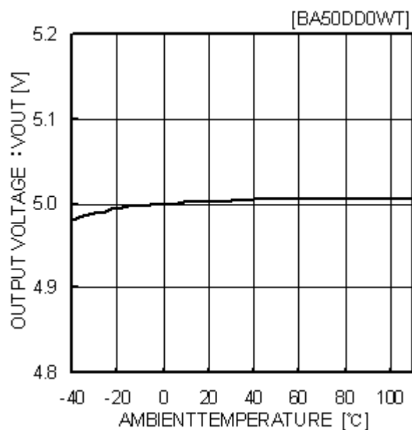
Fig.21 Temperature Characteristics
