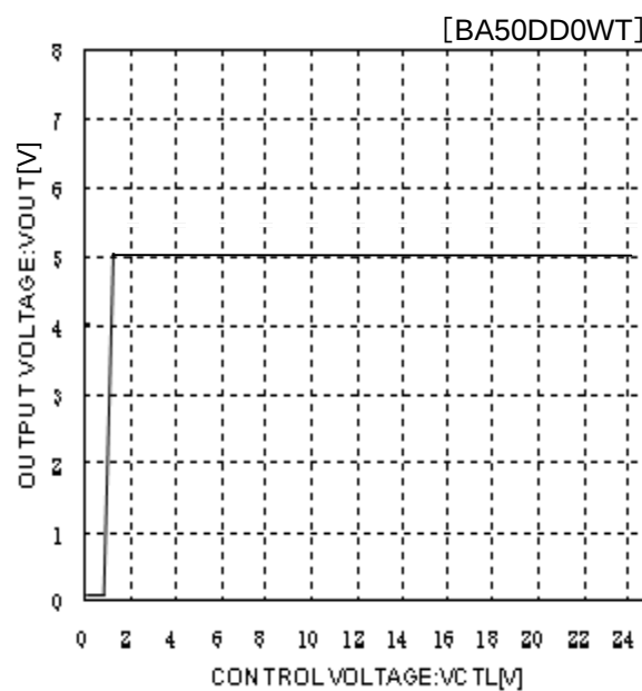
Fig.24 CTL Voltage vs. Output Voltage
